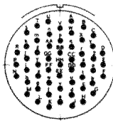
22-55 55 NO.20 CONTACTS
