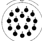
20-16 16 NO.16 CONTACTS
