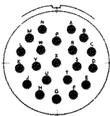
22-21 21 NO.16 CONTACTS
