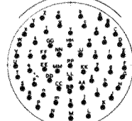
24-61 61 NO.20 CONTACTS
