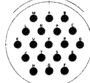
24-19 19 NO.12 CONTACTS
