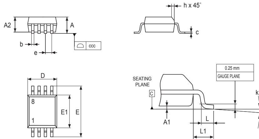
Figure 13. SO8N - Outline
