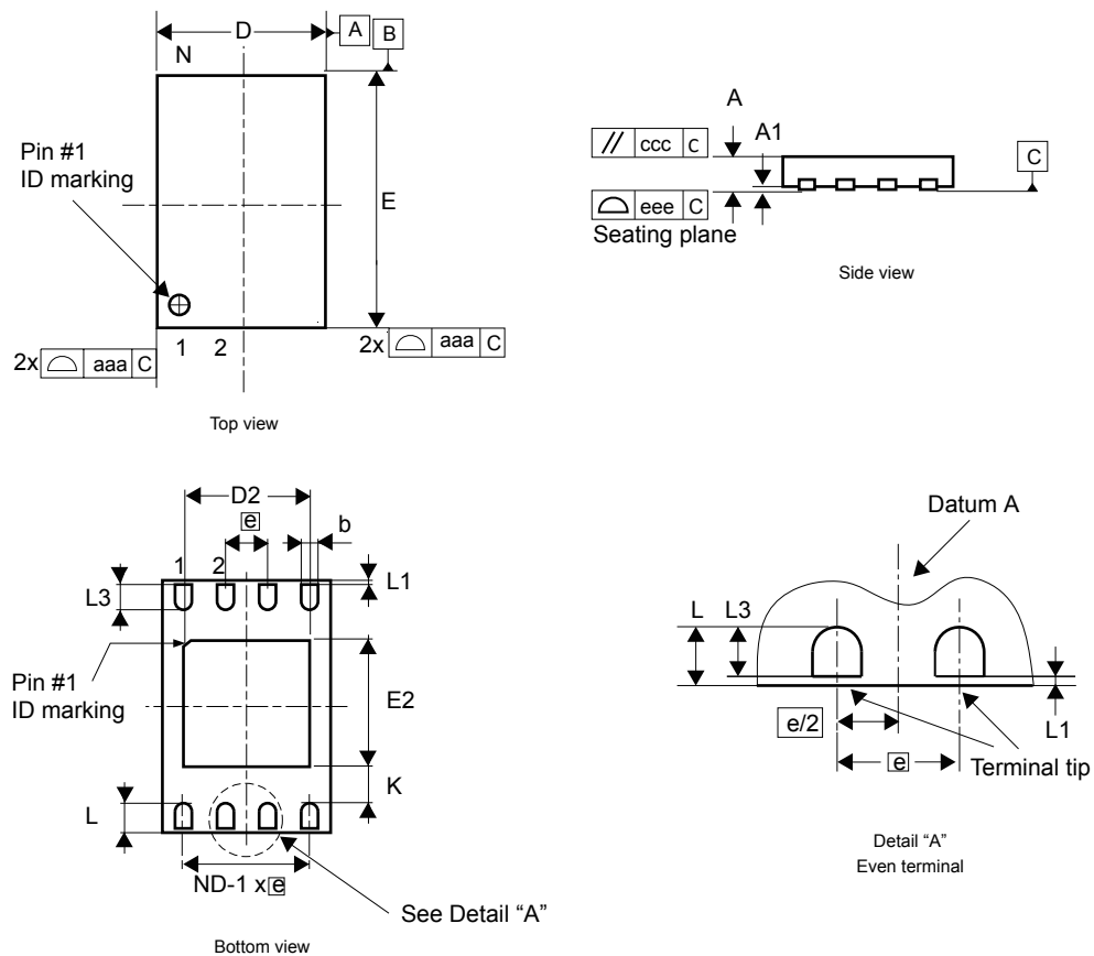
Figure 15. UFDFPN8 - Outline
