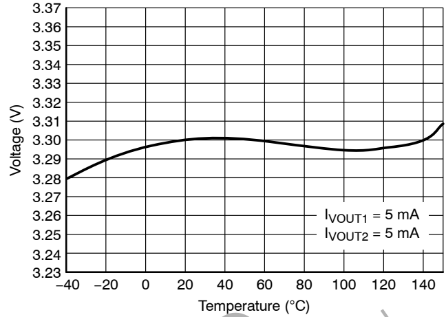
Figure 4. 3.3 V Output Voltage
