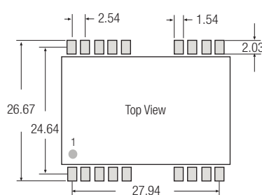
Pin area 0.1 x 0.50 0.50 23.40 Bottom View 1 2 3 4 5 9 10 11 12 24 23 22 21 20 16 15 14 13 11 x 2.54
