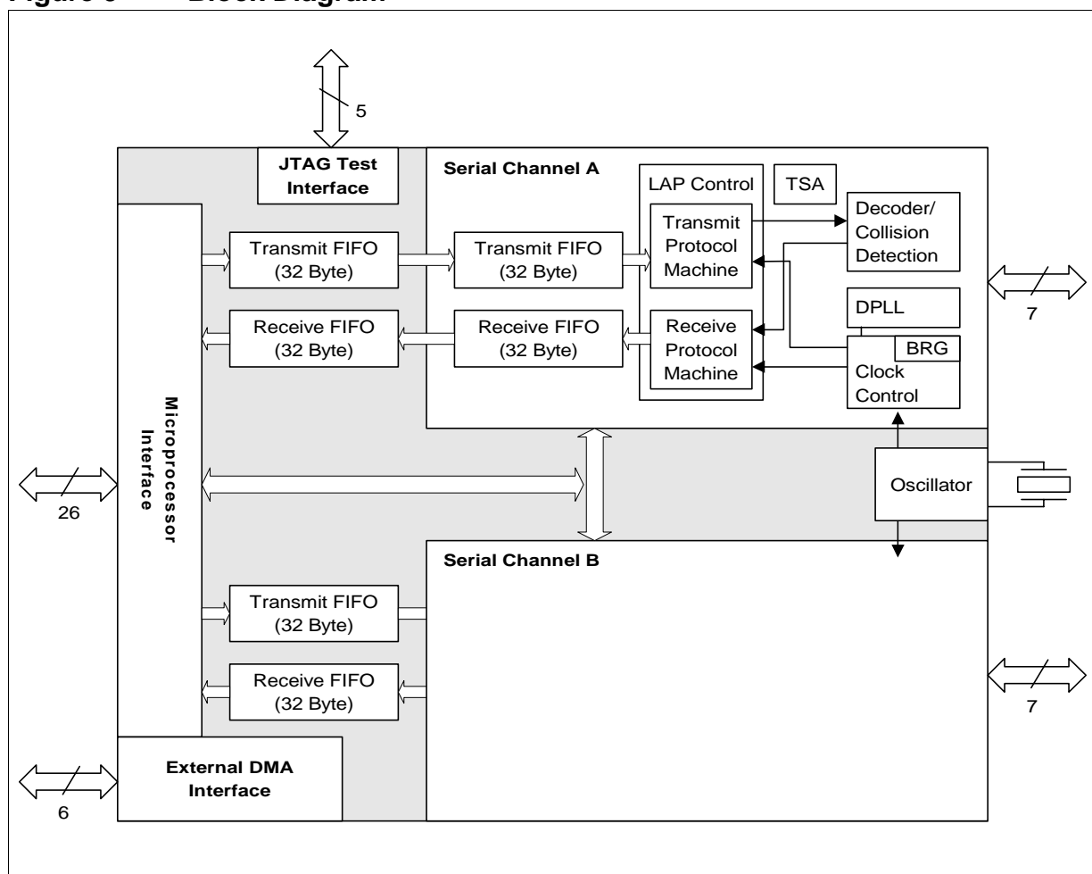
Figure 9 Block Diagram
