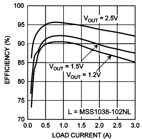
Efficiency vs. Load Current ( V_{IN} = 3.3\text{V} , f_{SW} = 1.5\ \text{MHz} )
