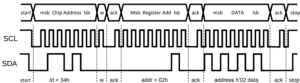
Figure 20. Write Cycle
