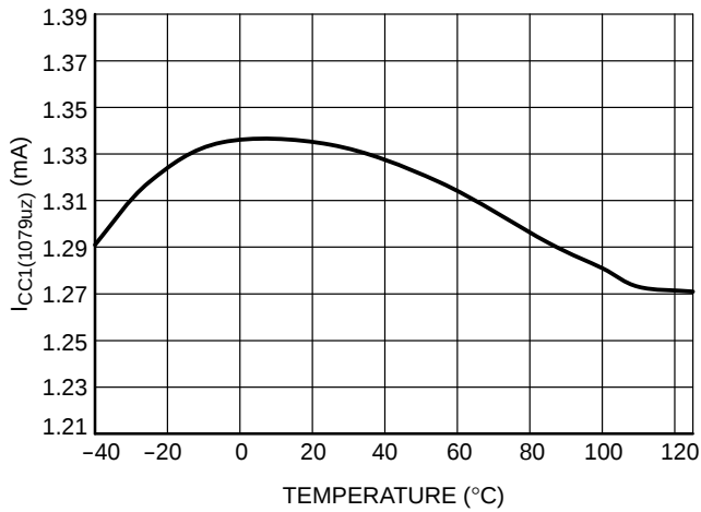
Figure 11. I_{CC1(0)1079\mu z} vs. Temperature
