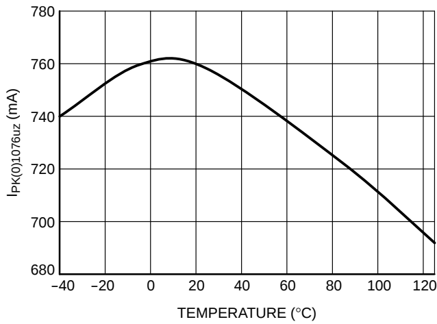
Figure 13. I_{PK(0)1076\mu z} vs. Temperature
