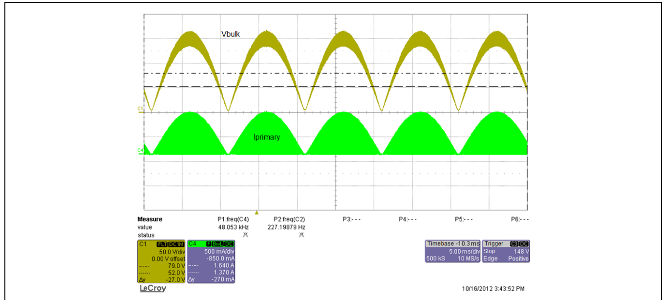
Figure 2.3 Active PFC
