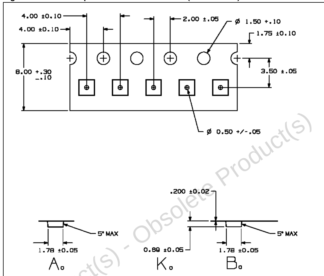
Figure 13. Carrier tape information for SOT-665 (1.6 x 1.6 mm)
