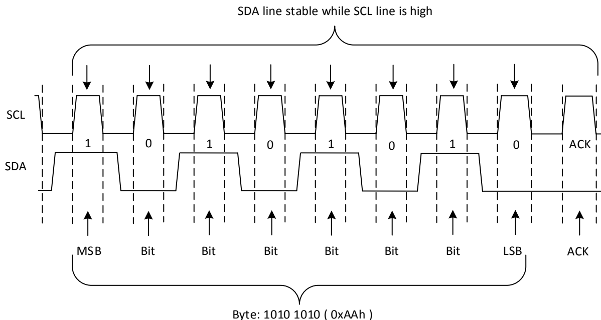
Figure 22. Bit Transfer
