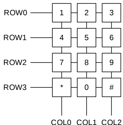
Figure 30. Example Keypad
