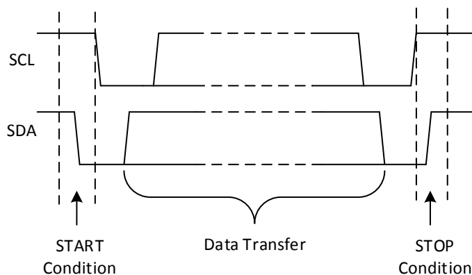
Figure 21. Definition of Start and Stop Conditions
