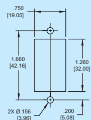
Panel Mounting Detail Mounting Detail Tolerance: ±.005 [0.13] unless noted
