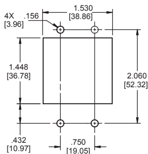
Panel Mounting Details Single Pole
