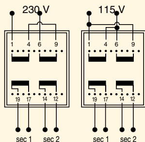
Possible primary connections
