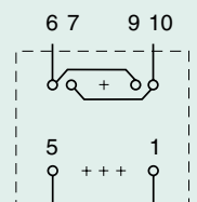
Recommended layout for transformers with 1 secondary winding (Allows the use of a transformer with 2 secondary windings)
