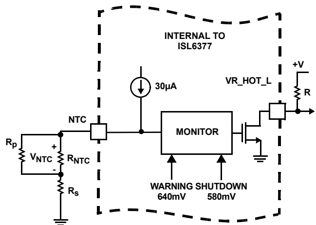
FIGURE 18. CIRCUITRY ASSOCIATED WITH THE THERMAL MONITOR FEATURE OF THE ISL6377
