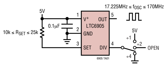
Basic Connection
