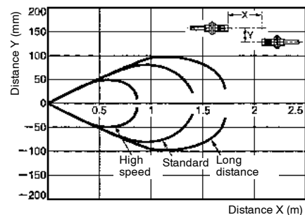
E32-TC200+E39-F1 with E3X-DAN amplifier (Through-beam)
