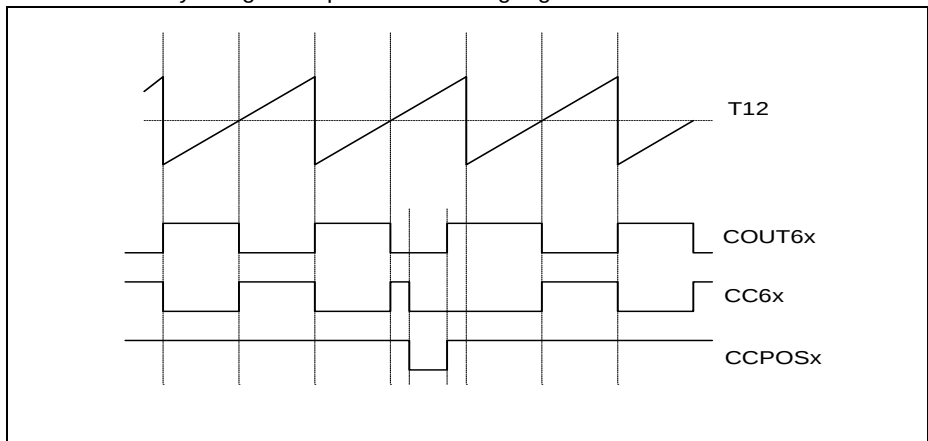
Figure 20 Hysteresis-like control mode
