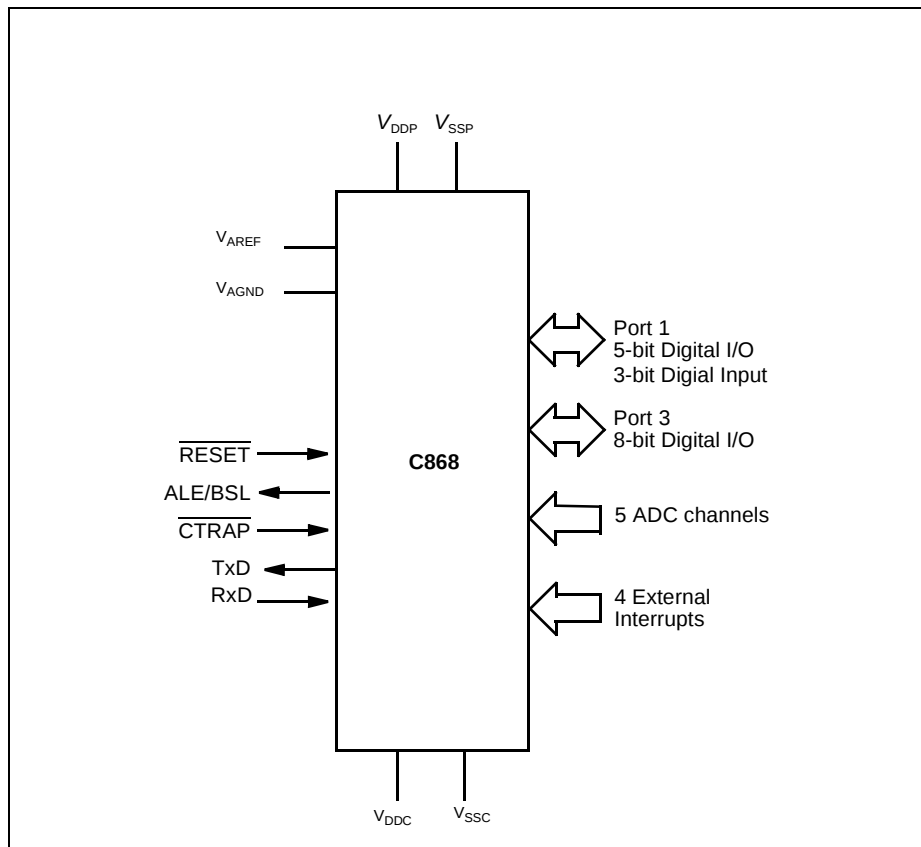
Figure 2 Logic Symbol
