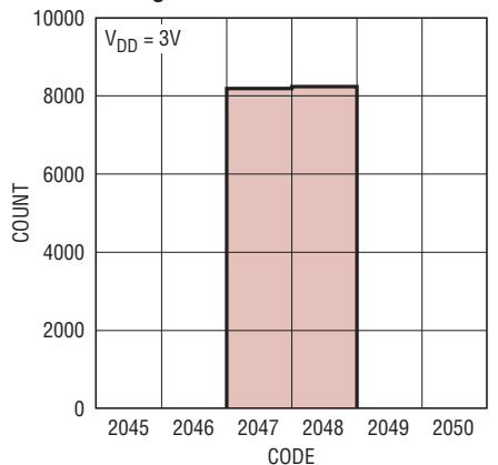
Histogram for 16384 Conversions
