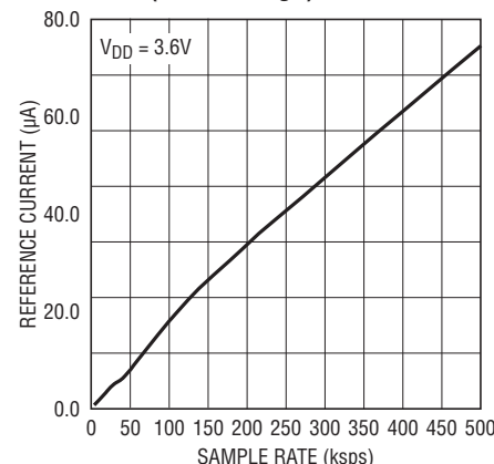
Reference Current vs Sample Rate (TS8 Package)
