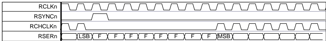
Figure 11-23. E1 Receive-Side RCHCLKn Gapped Mode During Channel 1
