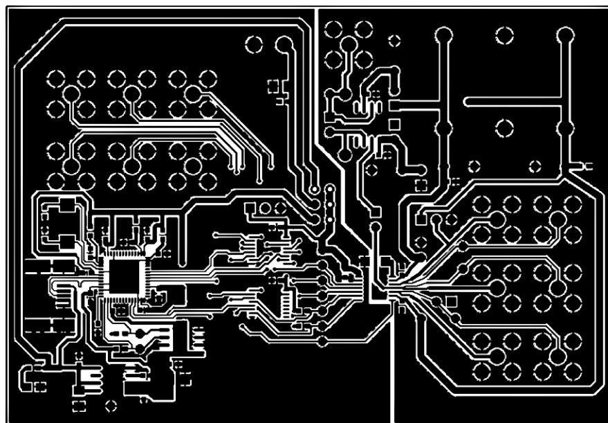
Figure 9. Component Side PCB Drawing
