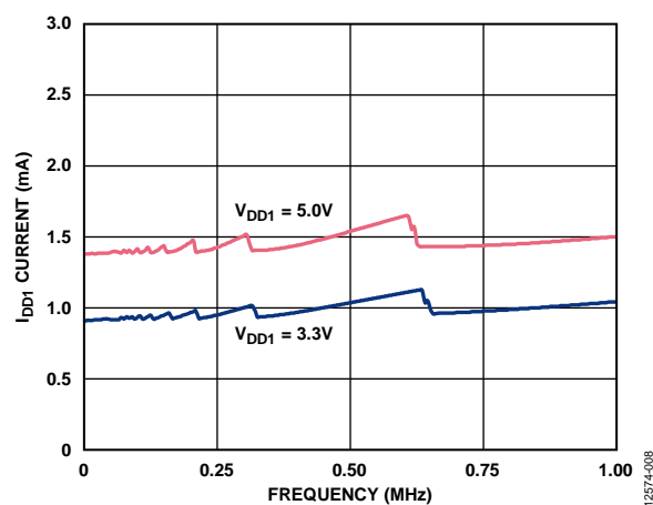
Figure 8. Typical I_{DD1} Current vs. Frequency
