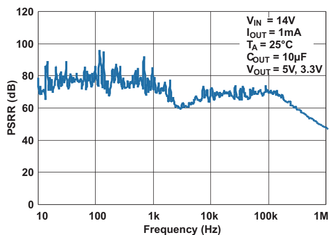
PSRR AT LIGHT LOAD CURRENT
