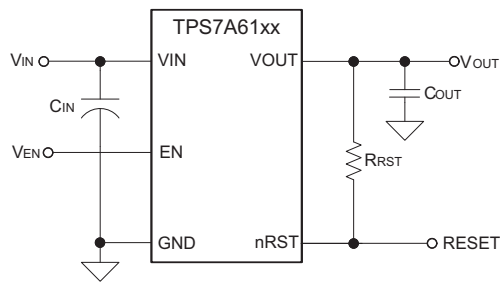
Figure 3. Enable Option
