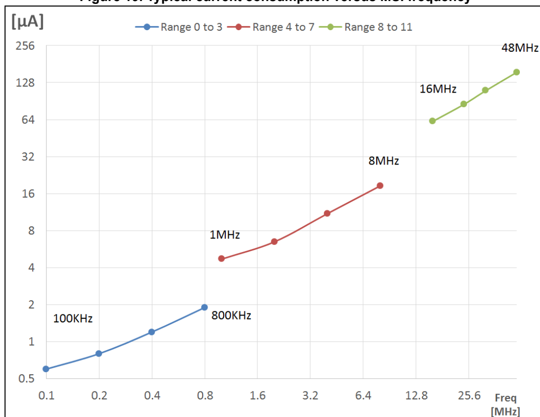
Figure 19. Typical current consumption versus MSI frequency
