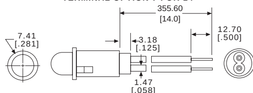
24 AWG WIRE LEADS - TERMINAL OPTION 3 FOR 6" WIRE LEADS TERMINAL OPTION 7 FOR 14"
