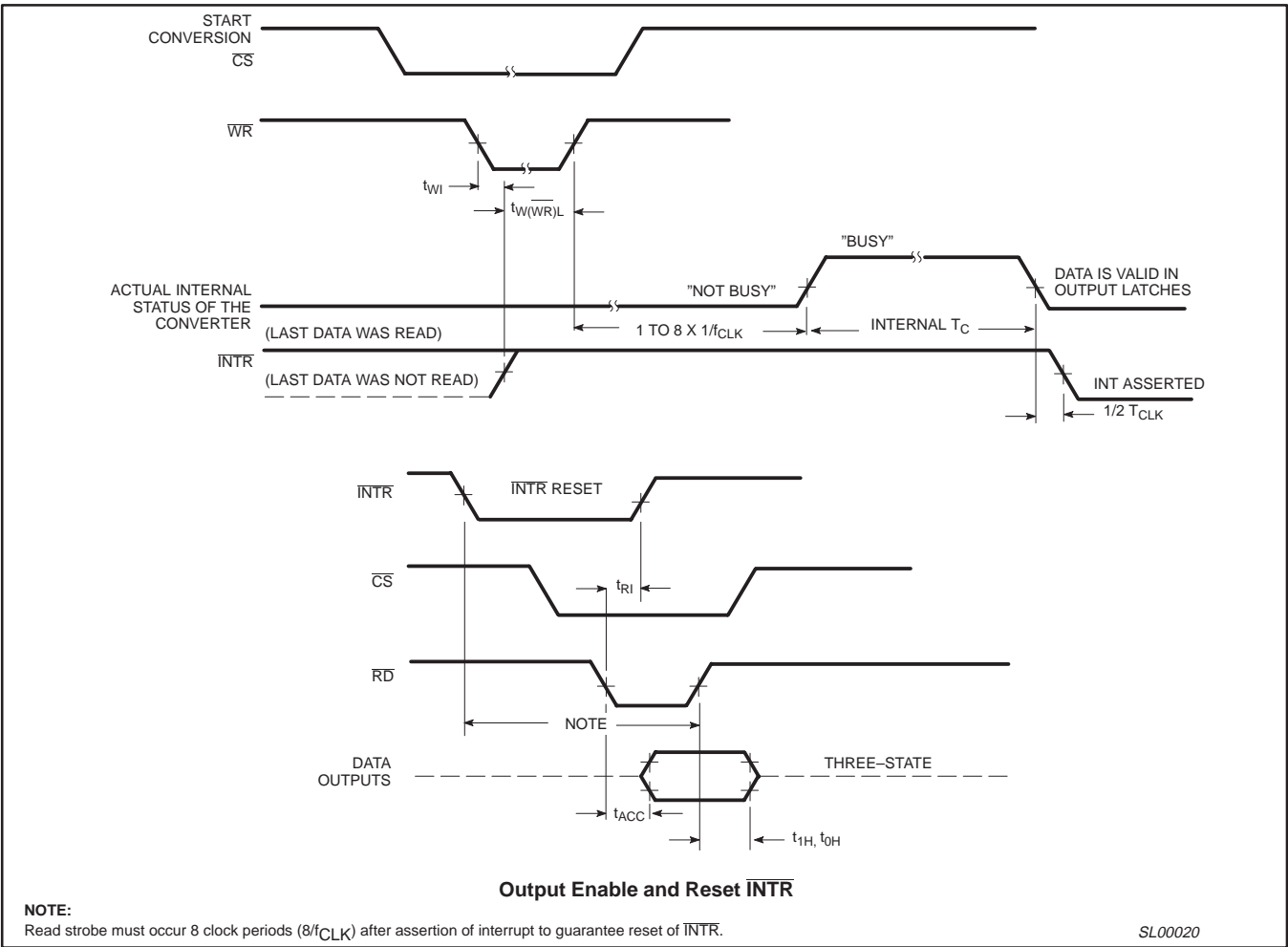
Figure 5. Timing Diagrams
