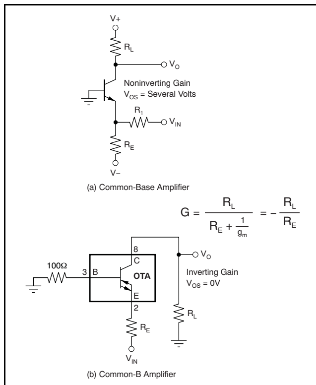
Figure 51. Common-Base Transistor vs Common-B OTA
