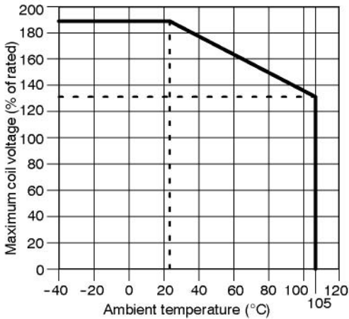
■ AMBIENT TEMPERATURE VS. MAXIMUM VOLTAGE
