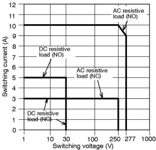
■ MAX. SWITCHING CAPACITY
