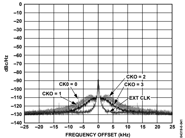
Figure 41. CLK Phase Noise vs. I BIAS Setting ( CKO ) (IF = 73.35 MHz, IF = 71.1 MHz, IFIN = -31 dBm, f CLK = 18 MHz, f REF = 16.8 MHz) (CLK SYN Settings: CKI = 7, CLR = 56, and CLN = 60 with f REF = 300 kHz)
