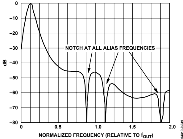
Figure 48. Signal Transfer Function of the Band-Pass \Sigma - \Delta Modulator from 0 f_{CLK} to 2f_{CLK}
