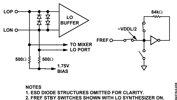
Figure 39. Equivalent Input of LO and REF Buffers
