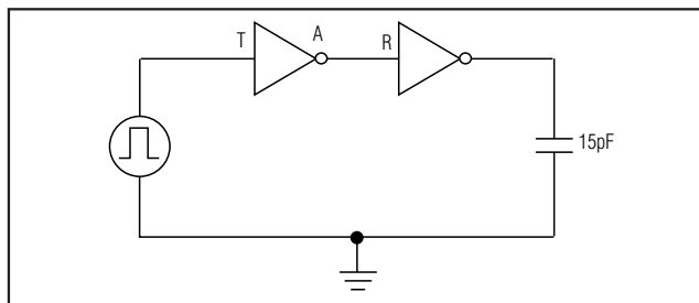
Figure 5. V.28 Receiver Test Circuit
