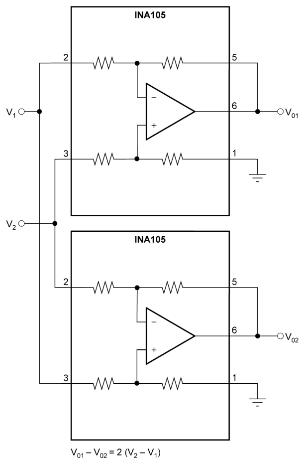
Figure 7-16. Differential Output Difference Amplifier
