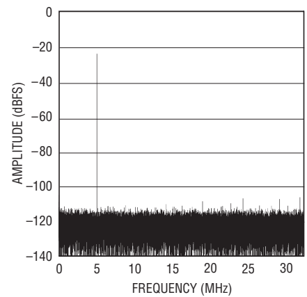
LTC2205: 64K Point FFT, f_{IN} = 5.1\text{MHz} , -25\text{dBFS} , PGA = 0, DITH = 0
