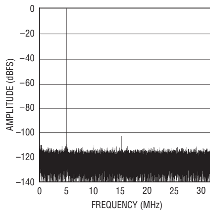
LTC2205: 64K Point FFT, 65Msps, f_{IN} = 5.1\text{MHz} , -1\text{dBFS} , PGA = 1, DITH = 0
