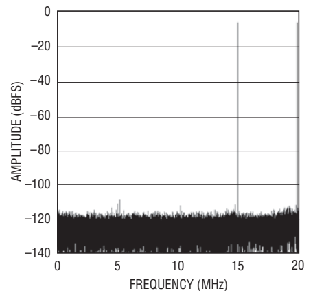
LTC2204: 64K Point FFT, f_{IN1} = 14.9\text{MHz} , -7\text{dBFS} , f_{IN2} = 20.1\text{MHz} , -7\text{dBFS} , PGA = 0, DITH = 0
