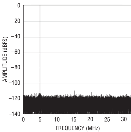
LTC2205: 64K Point FFT, f_{IN} = 5.1\text{MHz} , -1\text{dBFS} , PGA = 0, DITH = 0
