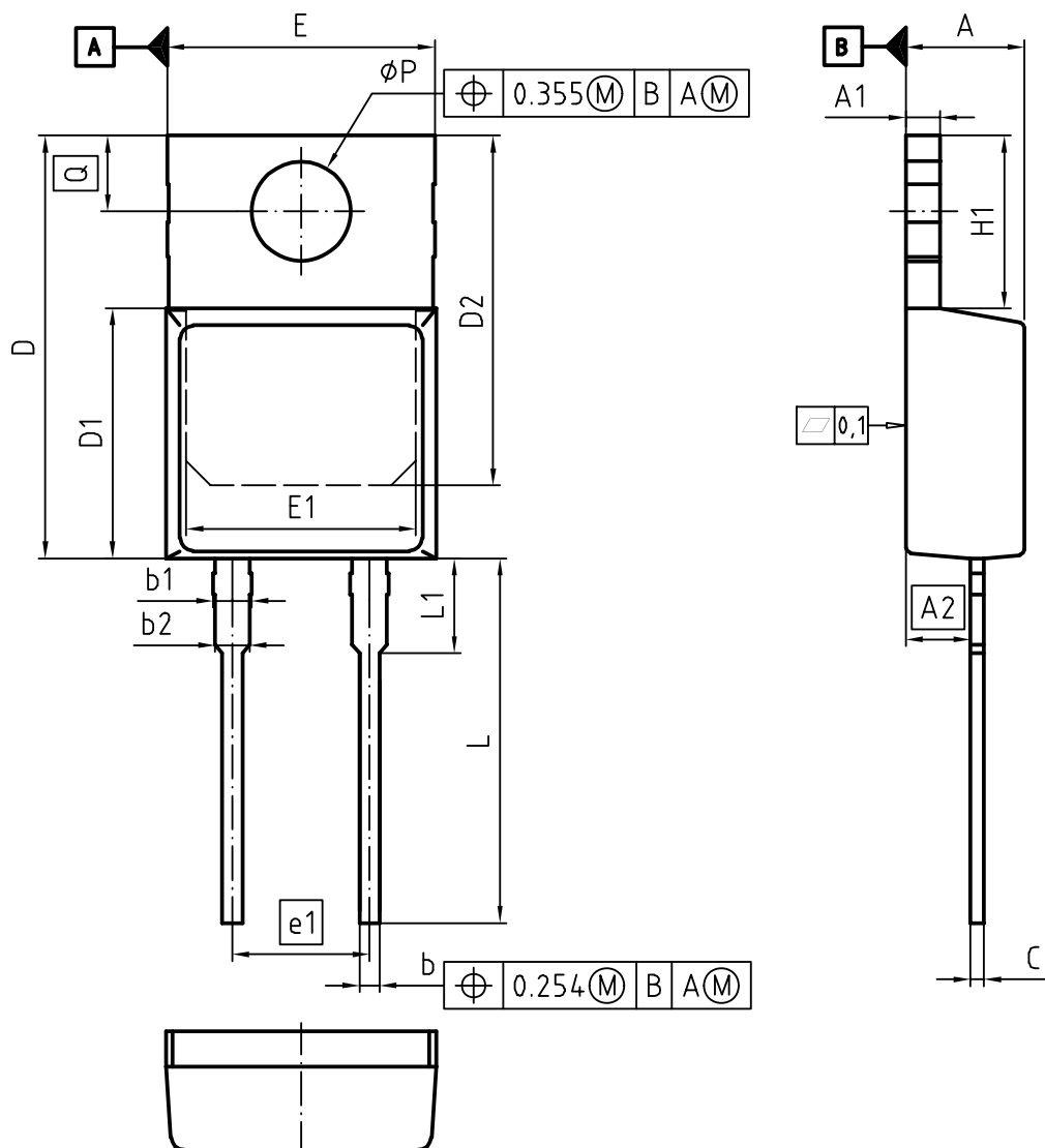
TO-220-2
