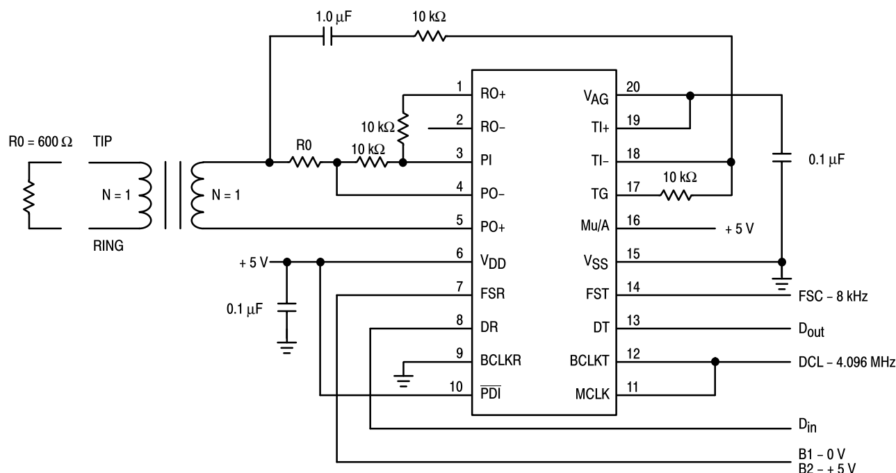
Figure 11. MC14LC5480 Transformer Interface to 600 \Omega Telephone Line with GCI Clocking
