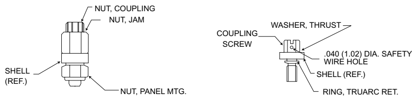
CORD-TO-CORD INSTALLATION
