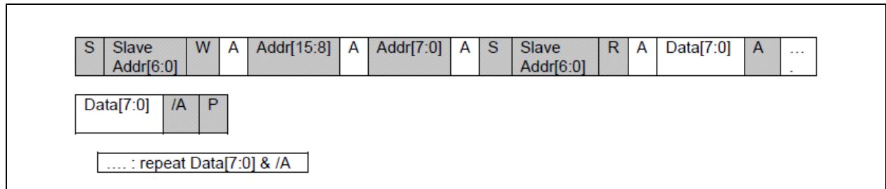
FIGURE 4-15: BURST REGISTER READ
