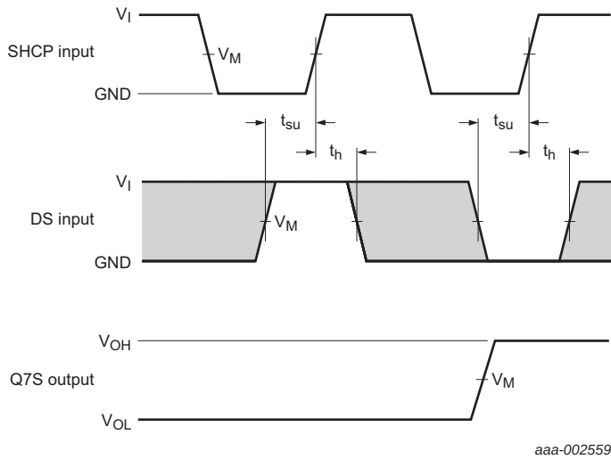
Measurement points are given in Table 8 . The shaded areas indicate when the input is permitted to change for predictable output performance. V OL and V OH are the typical output voltage levels that occur with the output load.
