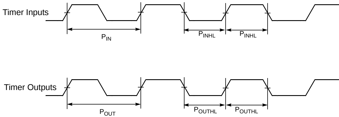
Figure 3-23 Timer Timing
