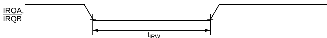
Figure 3-13 External Interrupt Timing (Negative-Edge-Sensitive)
