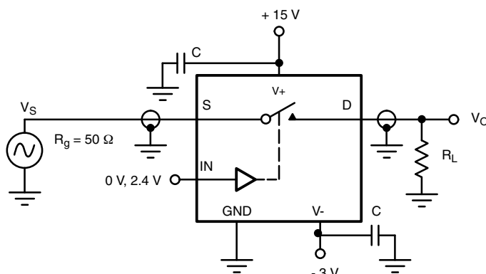
Figure 3. Charge Injection
