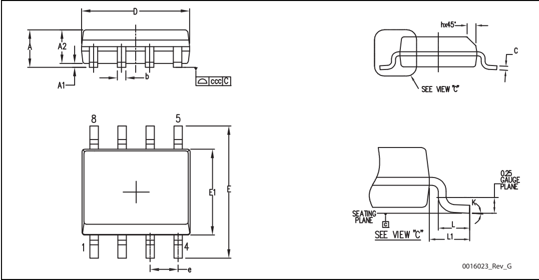
Figure 14. SO-8 drawings
