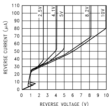
Figure 8-2. Reverse Characteristics and Minimum Operating Current
