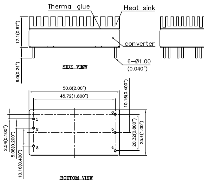
Mechanical Dimensions
