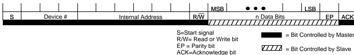
Figure 9. Read Transaction, master reads data from LM95010
