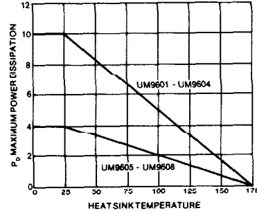
Power Rating
