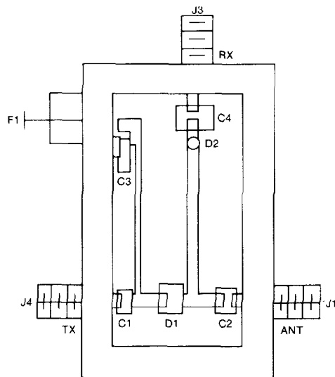
Assembly Drawing
