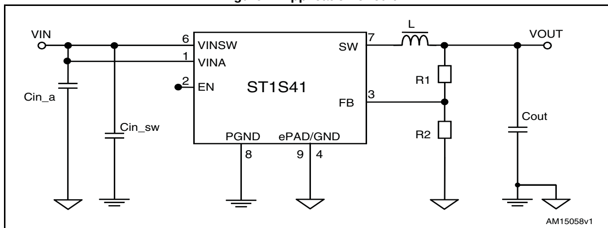
Figure 1. Application circuit
