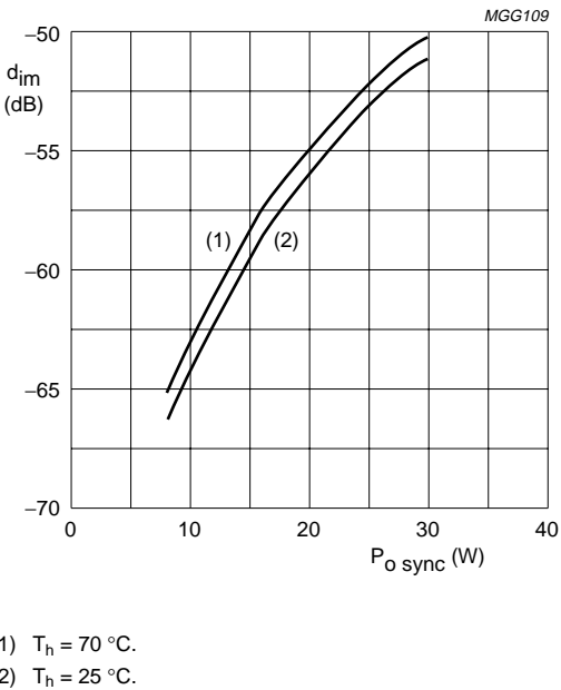
Fig.9 Intermodulation distortion as a function of peak synchronized output power.
