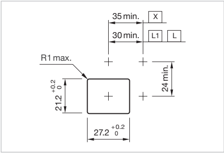
Mounting cut-outs [mm] L1 = Solder/Plug-in terminal 2.8 x 0.5 mm, L = Solder terminal, X = Screw terminal
