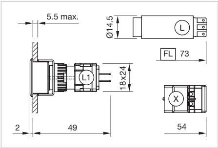
Dimensions [mm] L1 = Solder/Plug-in terminal 2.8 x 0.5 mm, L = Solder terminal, X = Screw terminal, FL = Flasher
