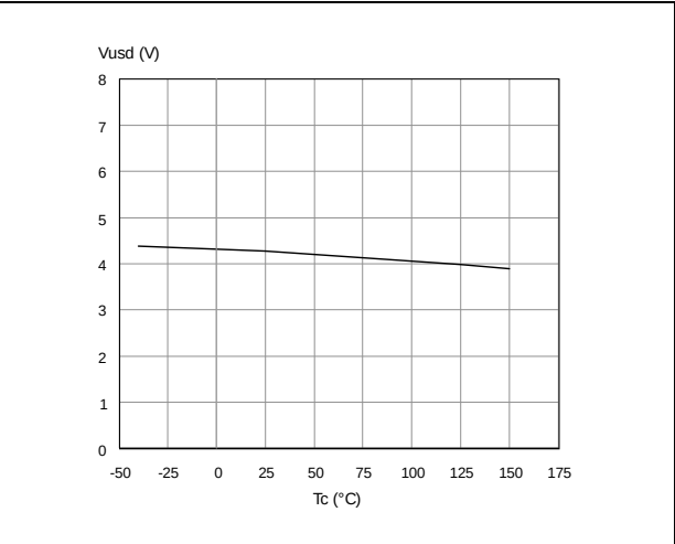
Figure 25. Undervoltage shutdown
