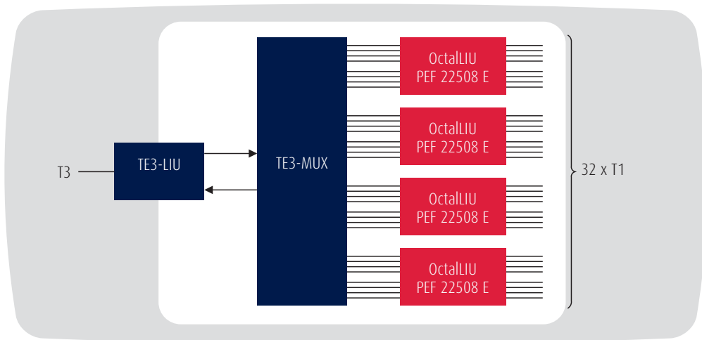
Application Example 32-Channel E1/T1/J1 Line Card with OctalLIU
