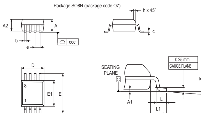
Figure 19. SO8N – Outline
