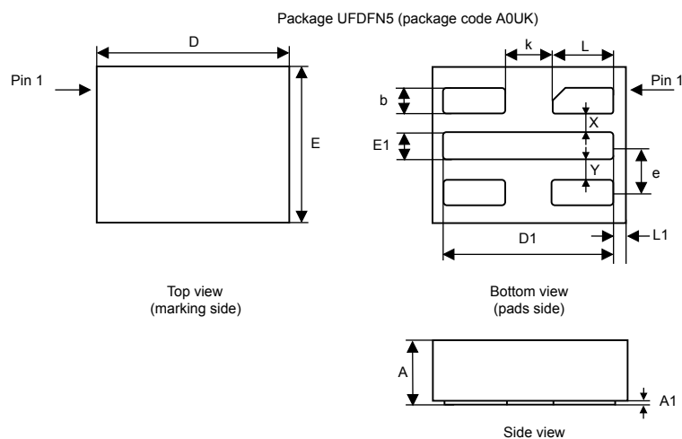
Figure 13. UFDFPN5 - Outline
