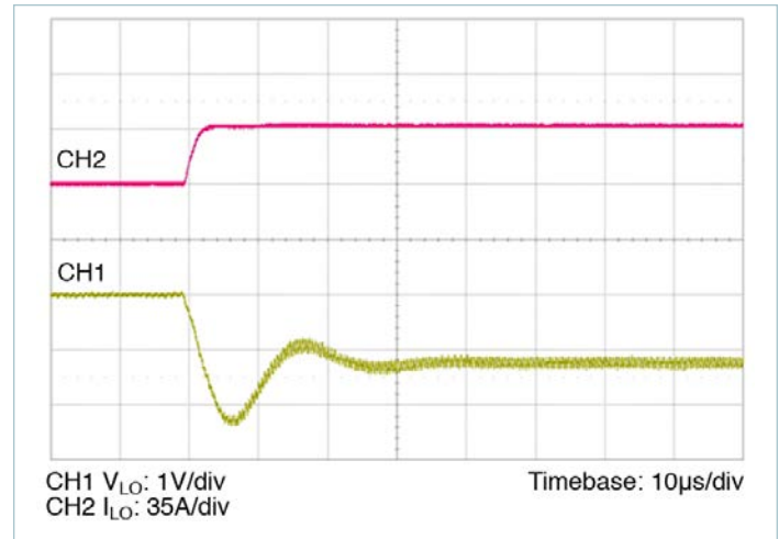
Figure 15 — 0 – 35A transient response: C_{HI\_IN\_EXT} = 10\mu F , no external C_{LO\_OUT\_EXT}
